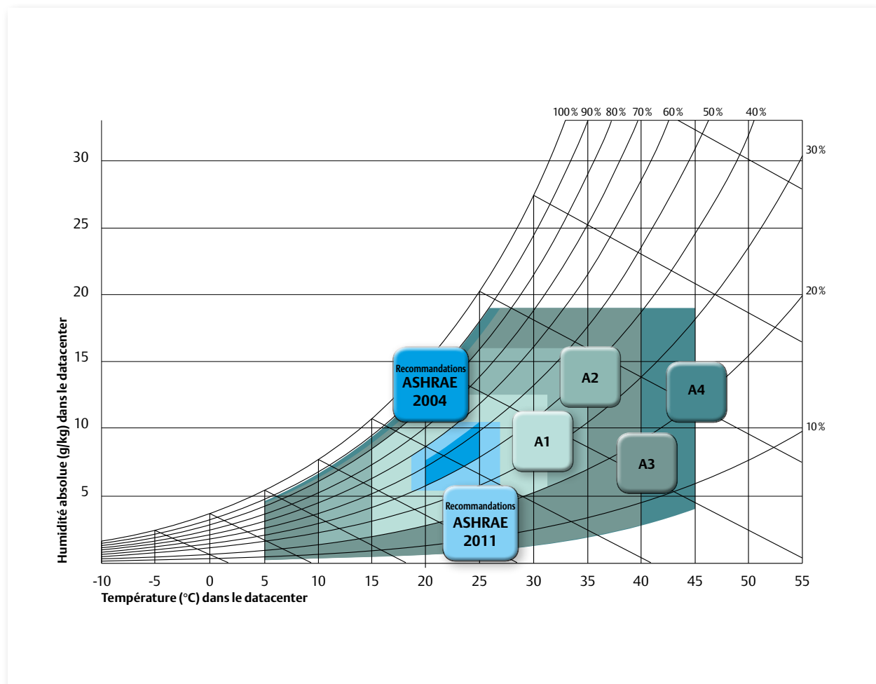
Figure 1. Recommandations ASHRAE
